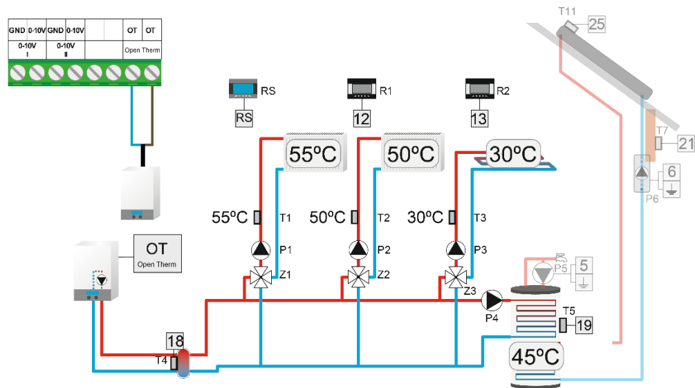
An example system controlled using the Open Therm protocol
